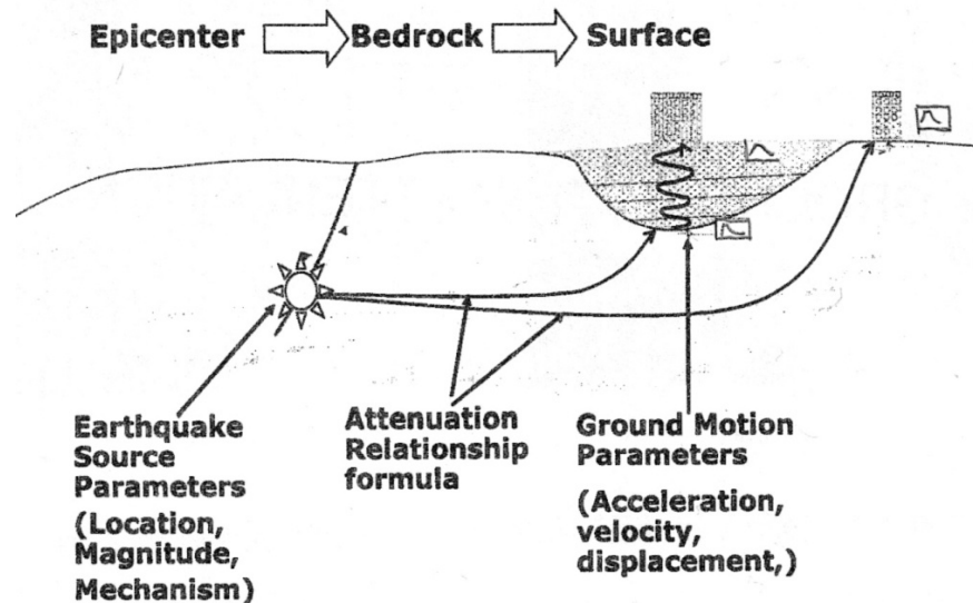
Figure 1.2 Schematic illustration of wave propagation through engineering bedrock and soil surface
